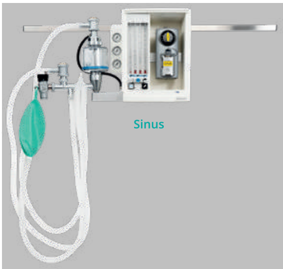
Compact circulation system
